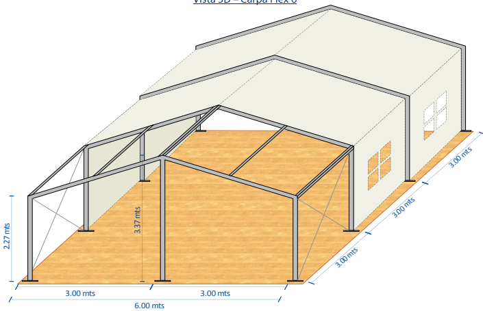
Vista 3D – Carpa Flex 6
