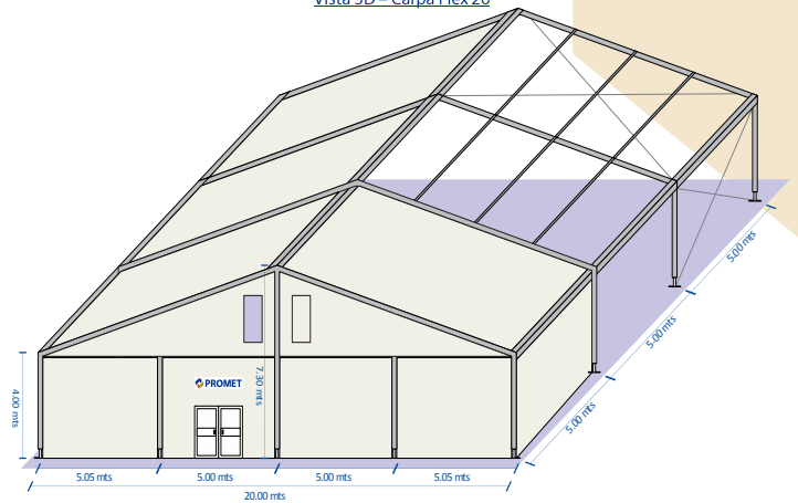
Vista 3D – Carpa Flex 20
